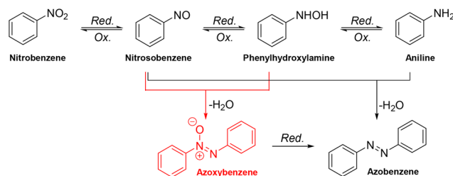
Fig. 1 General synthetic pathway for the formation of azoxybenzene/azobenzene from nitrobenzene.
