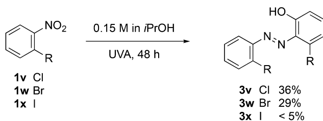
Fig. 4 Unexpected Wallach products of the attempted homocoupling of ortho -halonitrobenzenes.
