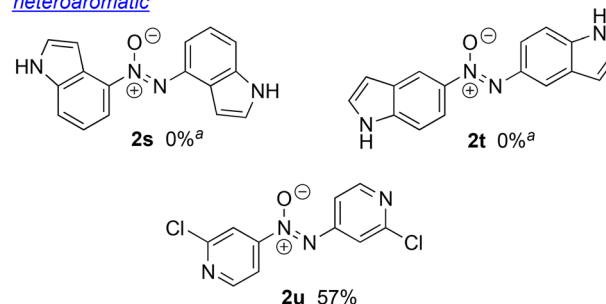
Fig. 3 Substrate scope for the synthesis of azoxybenzenes via reductive homocoupling of nitroarenes. The general procedure described above was applied. If not noted, reactions were irradiated for 48 hours. Yield reported as isolated yield after purification by column chromatography. The identity of each product was confirmed by 1 H NMR, 13 C NMR and GC-MS (see ESI † ). a Reaction irradiated for 24 hours.
