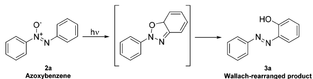
Fig. 2 Observed photo-Wallach rearrangement of azoxybenzene.
